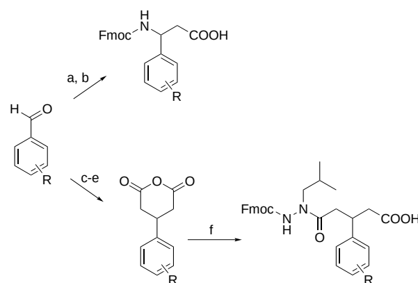
Scheme 1. a) \text{NH}_4\text{OAc} , malonic acid, EtOH, 80^\circ\text{C} ; b) Fmoc-Cl, \text{NaHCO}_3 , dioxane, 0^\circ\text{C} ; c) ethyl acetoacetate, piperidine, room temperature; d) KOH (20M), 85^\circ\text{C} ; e) acetic anhydride, 120^\circ\text{C} ; f) N -Fmoc- N' -isopropylhydrazine, THF, 70^\circ\text{C} .
